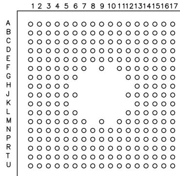
Figure 3. 256-ball BGA Pinout (Top View)
