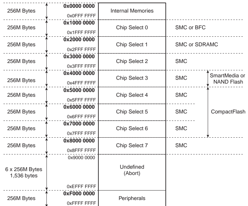
Figure 4. External Memory Mapping
