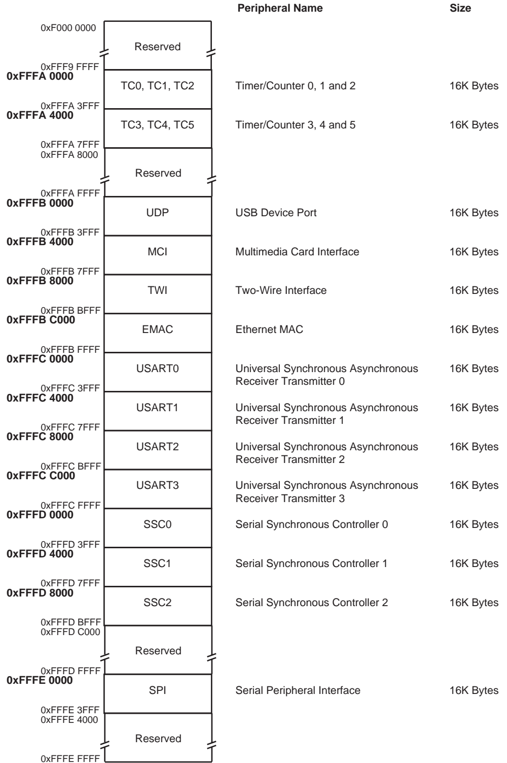
Figure 7. User Peripherals Mapping
