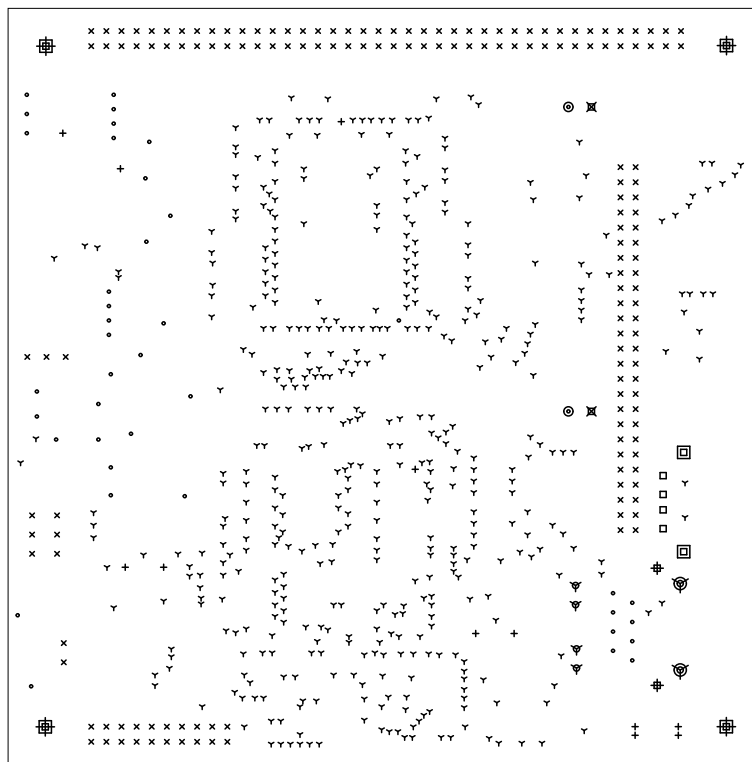
Board outline is the centerline of this 10 mil rectangle - 0,0 to 3940,3940 mls
